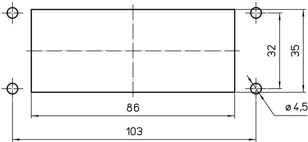
Panel cut-out
